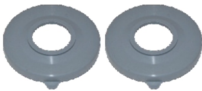
EK34 Dust Cover Ø32*Ø84*18mm
