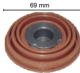
EK15/ET41 Tappet and Boot
